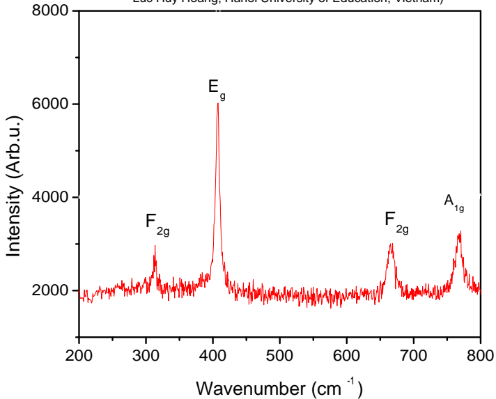
Raman spectra of natural spinel \text{MgAl}_2\text{O}_4 (Ex: 514.5 nm, T64000 MicroRaman Luc Huy Hoang, Hanoi University of Education, Vietnam)
